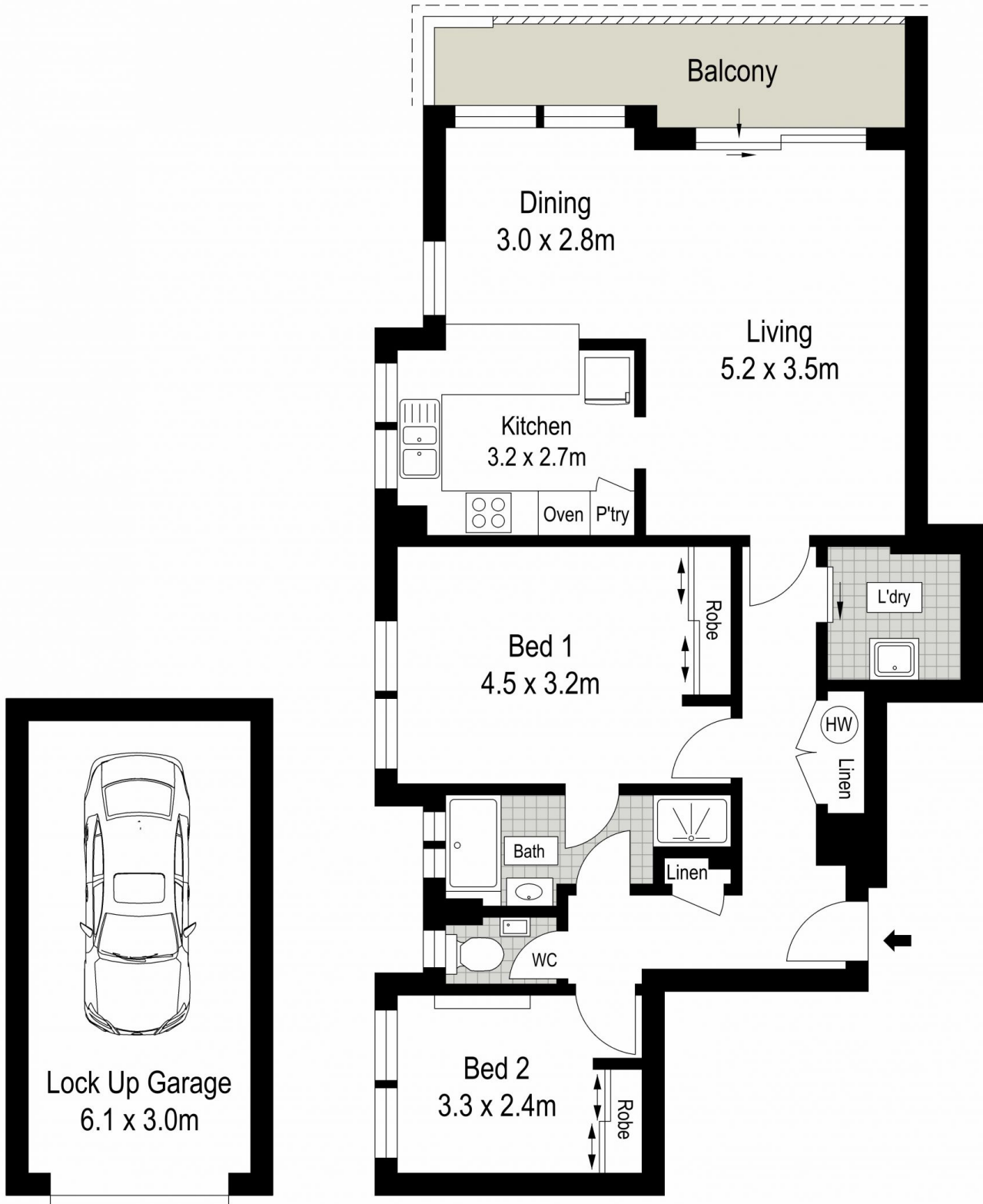
GROUND FLOOR
